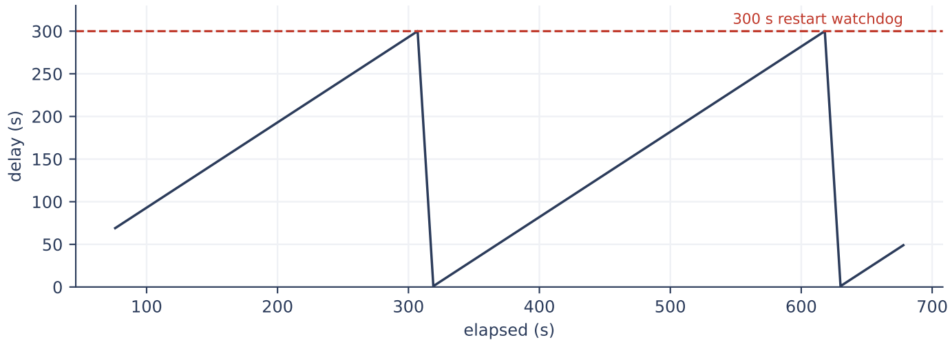
NTRIP correction delay vs 300 s restart (RTK25) — corrections are marginal
